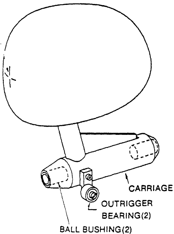
FIGURE 9a - HEADFORM & SUPPORT ASSEMBLY
