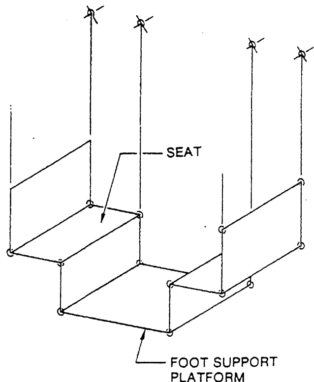
FIGURE 3 - FOOT SUPPORT INTENDED TO SUPPORT BOTH FEET
