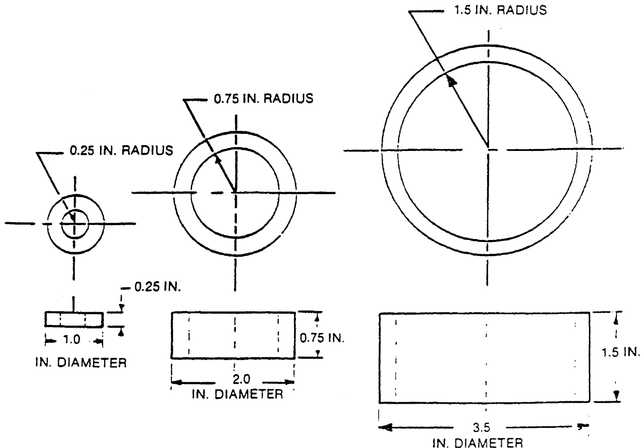
FIGURE 5 - PROTRUSION TEST GAUGES
