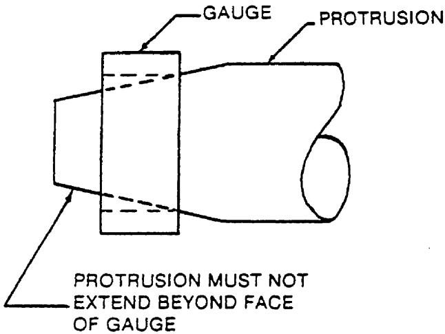
FIGURE 6 - PROTRUSION TEST
