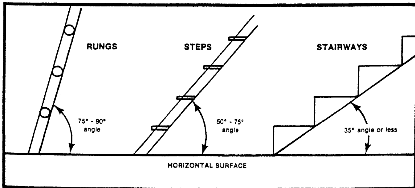
FIGURE 5 (SIDE VIEW)
