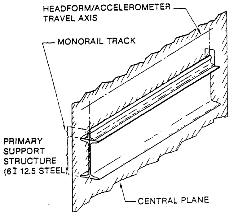
FIGURE 9 - IMPACT TEST SET-UP
