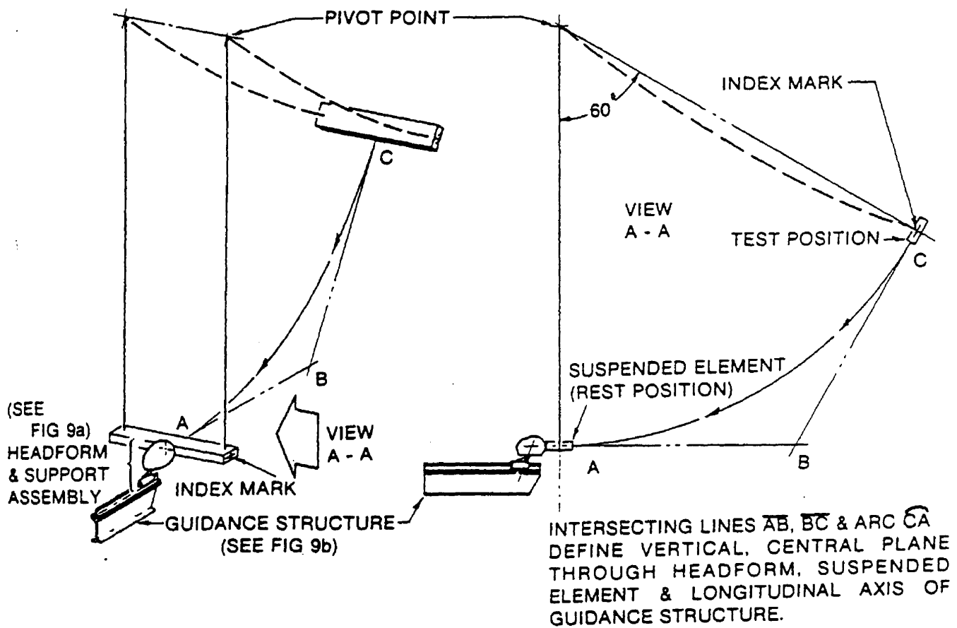
FIGURE 9 - IMPACT TEST SET-UP
