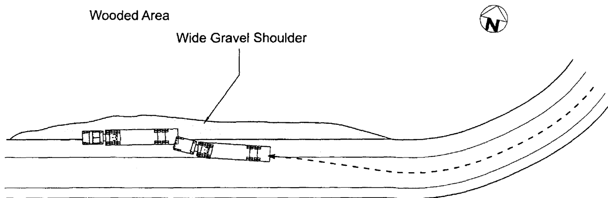
Figure 6. Case Study 1: Crash Diagram, Suburban Interstate Ramp
