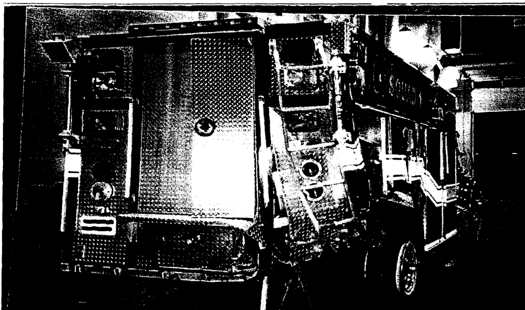
Figure 15. Case Study 3: View Looking at Rear of Involved Fire Truck Showing Damage to Right Corner
