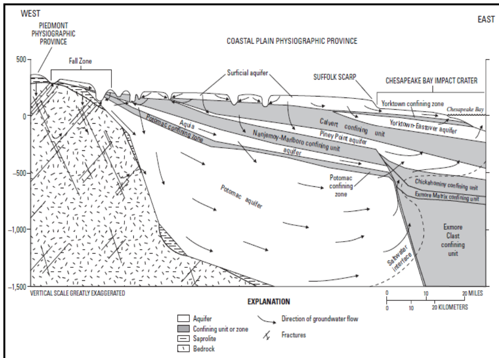
Figure 9: Generalized hydrogeologic section and directions of ground-water flow in the Virginia Coastal Plain (from Figure 2 of MFarland, E.R., and Bruce, T.S., 2006, The Virginia Coastal Plain Hydrogeologic Framework: U.S. Geological Survey Professional Paper 1731 , 118 p., 25 pls.; altitudes relative to National Geodetic Vertical Datum of 1929).
