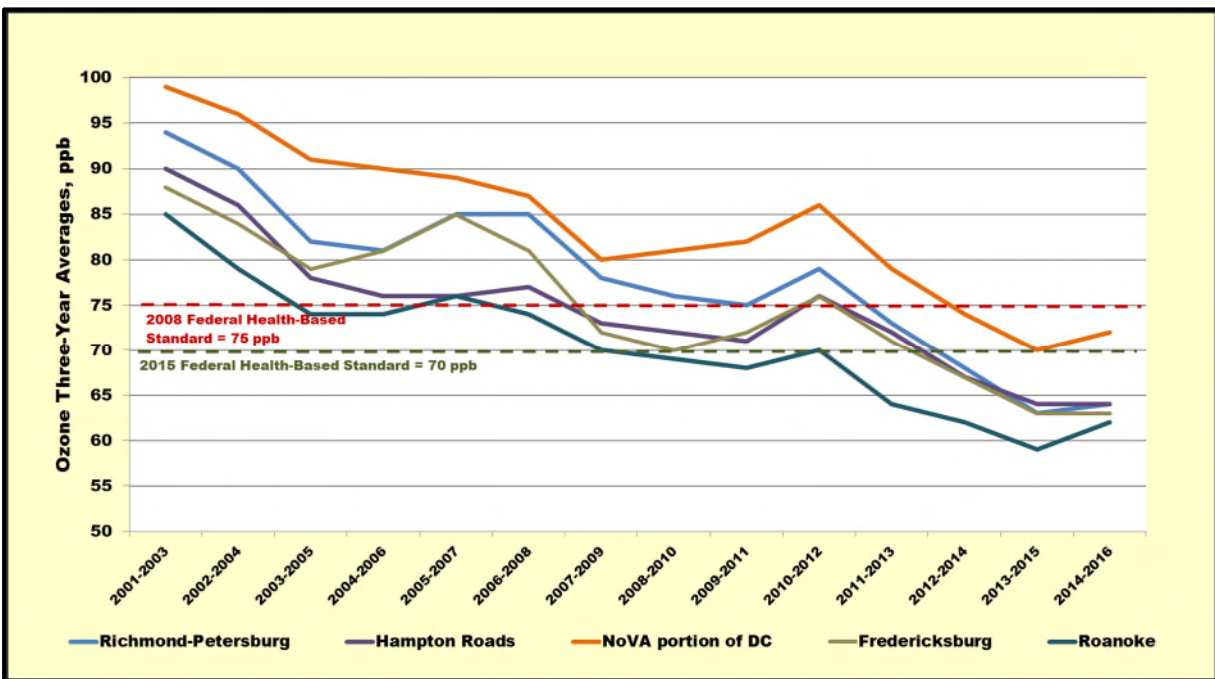
Figure 2-2: Ozone Concentrations
