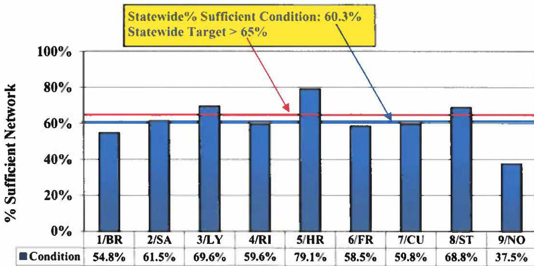
Figure 9: Percent Sufficient Pavements: Statewide and by District – Secondary (2017)
