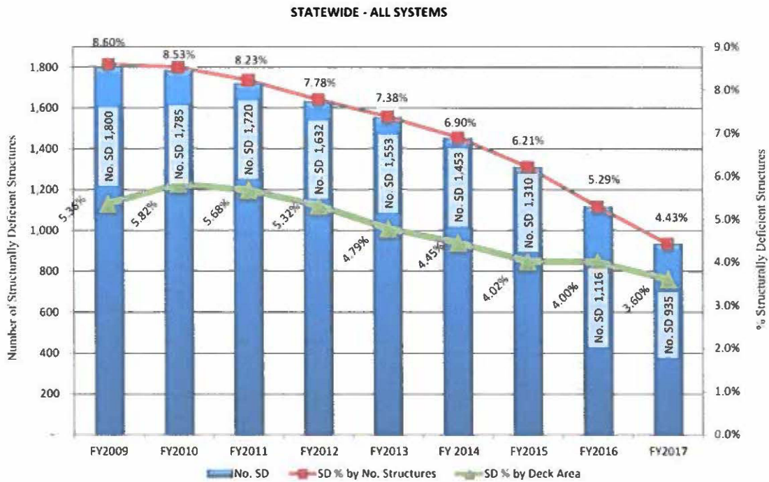
Figure 12: Percentage of and Number of Structurally Deficient Structures
