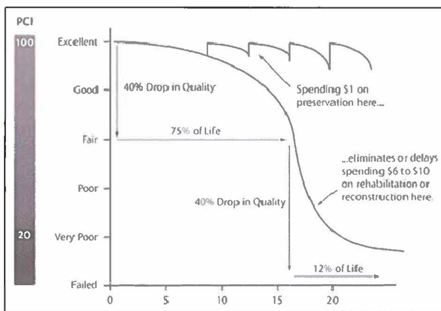
Figure 40: Impact of Maintenance Timing on Asset Condition
