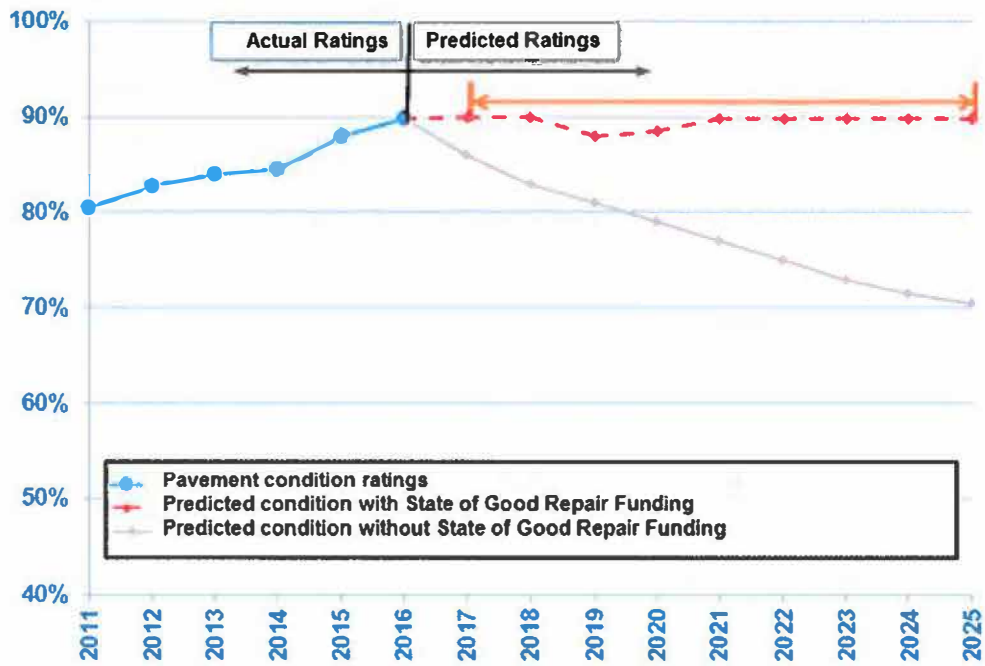
Figure 32: Previous and Forecasted Pavement Condition (Percent Sufficient) – Interstate
