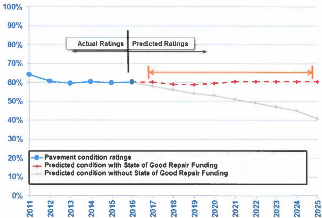
Figure 34: Previous and Forecasted Pavement Condition (Percent Sufficient) – Secondary
