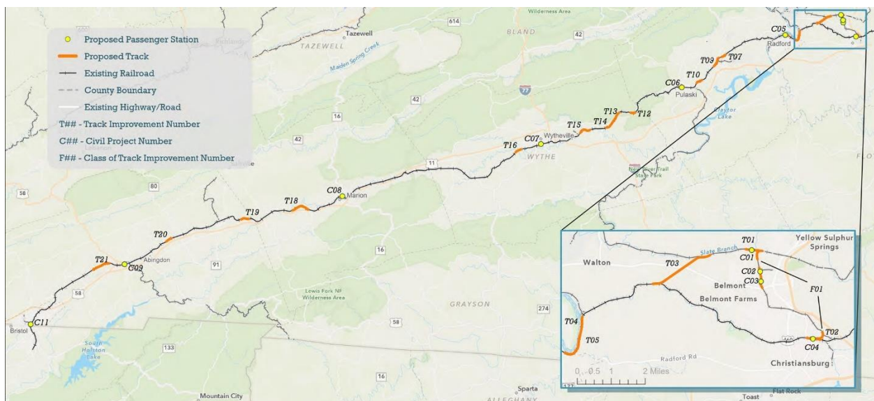
FIGURE 2.3: PROPOSED TRACK IMPROVEMENTS
