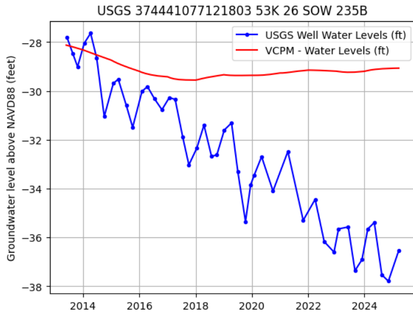
Figure 3. USGS Regional Observation Well 53K 26 SOW 235B, Potomac Aquifer water levels (Patapsco Formation) recorded from 2013 to present (well depth 320.7 ft bls, land surface 162.95 ft msl) and VAHydroGW-VCPM reported use water levels.
