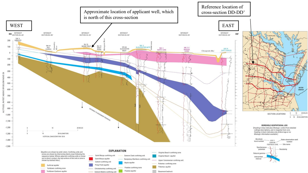
Coastal Plain (2006) Cross-Section DD-DD' from USGS Professional Paper 1731.
