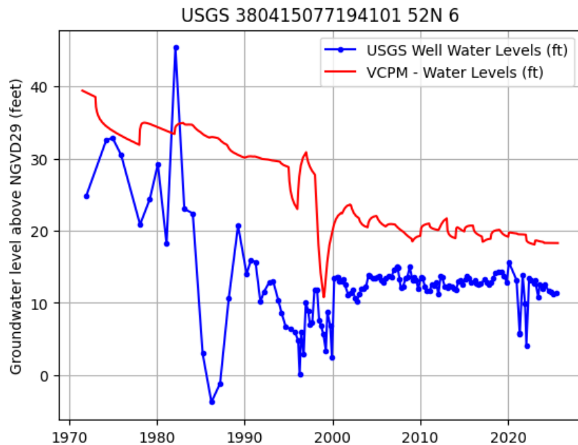
Figure 3. USGS Regional Observation Well 52N 6, Potomac Aquifer water levels (Patuxent Formation) recorded from 1971 to present (well depth 500.0 ft bls, land surface 204.0 ft msl) and VAHydroGW-VCPM reported use water levels.
