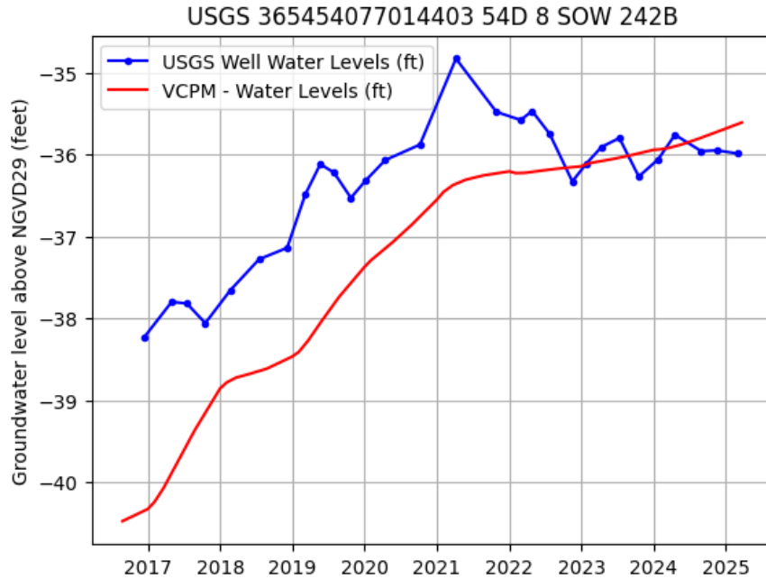
Figure 2. USGS Regional Observation Well 54D 8 SOW 242B, Potomac Aquifer water levels (Patapsco Formation) recorded from 2016 to present (well depth 480.0 ft bls, land surface 93.0 ft msl) and VAHydroGW-VCPM reported use water levels.
