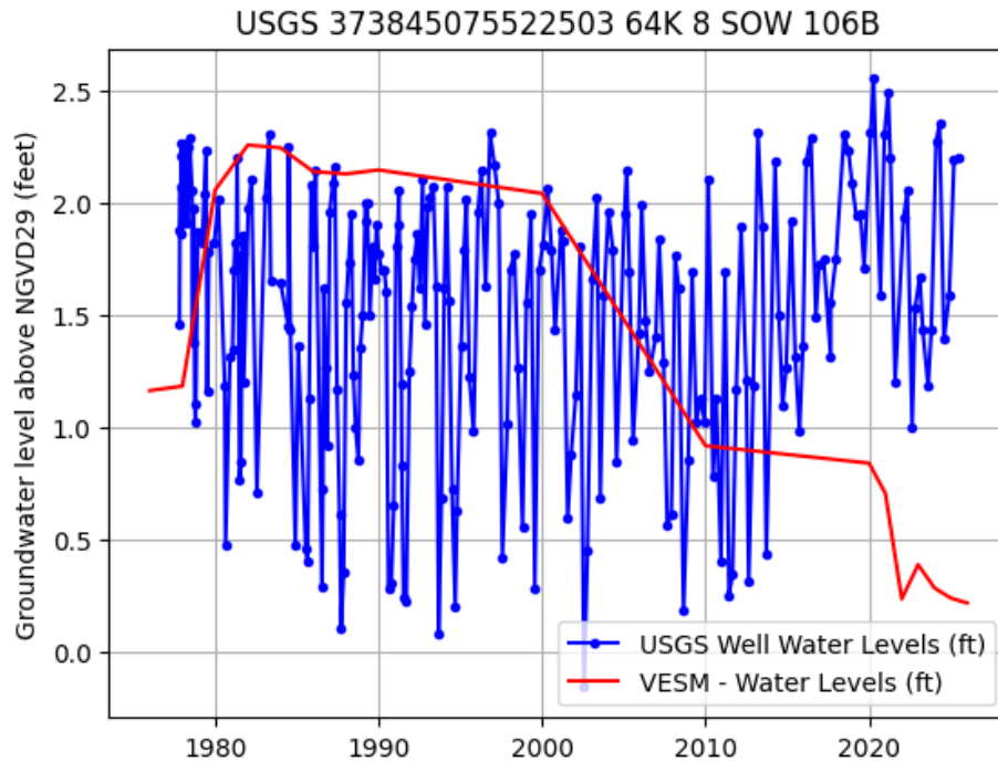
Figure 2. USGS Regional Observation Well 64K 8 SOW 106B, Upper Yorktown-Eastover aquifer water levels recorded from 1977 to present (well depth 95.0 ft bsl, land surface 3.0 ft msl) and VAHydroGW-VESM reported use water levels.
