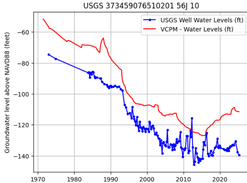
Figure 2. USGS Regional Observation Well 56J 10, Potomac Aquifer water levels (Upper Cretaceous Series) recorded from 1972 to present (well depth 437.0 ft bls, land surface 101.4 ft msl) and VAHydroGW-VCPM reported use water levels.
