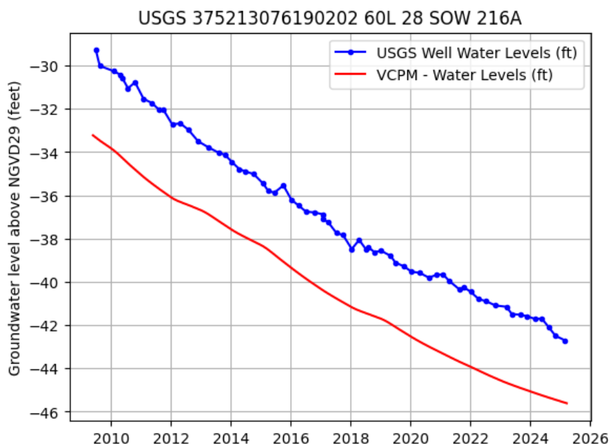
Figure 3. USGS Regional Observation Well 60L 28 SOW 216A, Potomac Aquifer water levels (Patapsco Formation) recorded from 2009 to present (well depth 1224.0 ft bls, land surface 110.0 ft msl) and VAHydroGW-VCPM reported use water levels.
