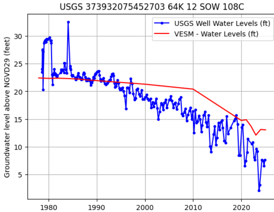
Figure 4. USGS Regional Observation Well 64K 12 SOW 108C, Lower Yorktown-Eastover aquifer water levels recorded from 1978 to present (well depth 284.0 ft bls, land surface 47.0 ft msl) and VAHydroGW-VESM reported use water levels.
