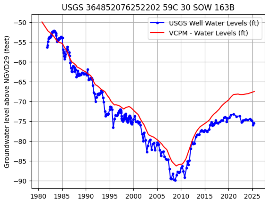
Figure 2. USGS Regional Observation Well 59C 30 SOW 163B, Potomac Aquifer water levels (Patapsco Formation) recorded from 1981 to present (well depth 948.0 ft bls, land surface 15.0 ft msl) and VAHydroGW-VCPM reported use water levels.
