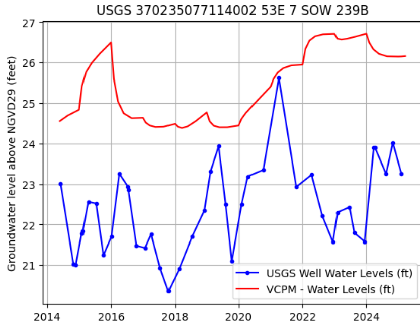
Figure 3. USGS Regional Observation Well 53E 7 SOW 239B, Potomac Aquifer water levels (Patapsco Formation) recorded from 2014 to present (well depth 290.0 ft bls, land surface 121.0 ft msl) and VAHydroGW-VCPM reported use water levels.
