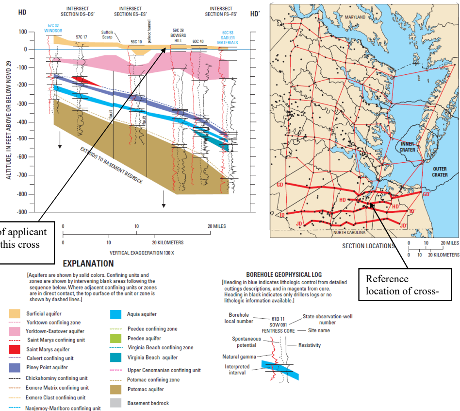
Coastal Plain (2006) Cross Section HD-HD' from USGS Professional Paper 1731.
