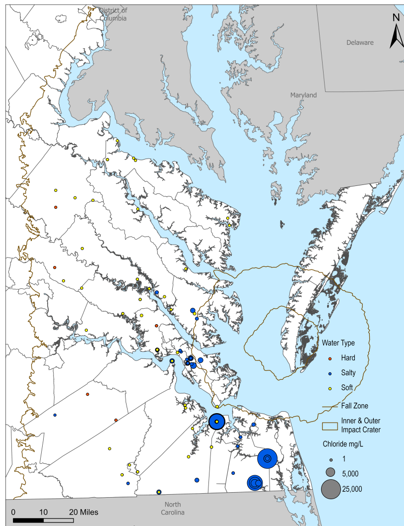
(b) Potomac aquifer groundwater quality samples 2007–2024.
