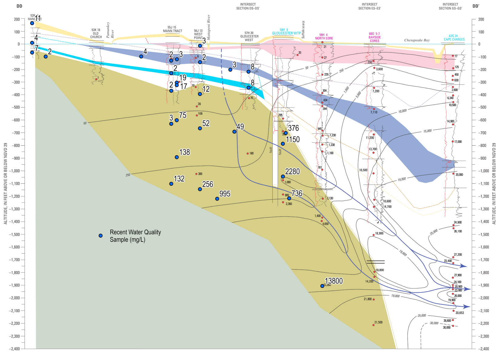
Figure 43: DD to DD' cross-section from McFarland (2010) and shown in Figure 40b, superimposed with select water-quality sample chloride concentrations from 2007–2024 (blue circles).
