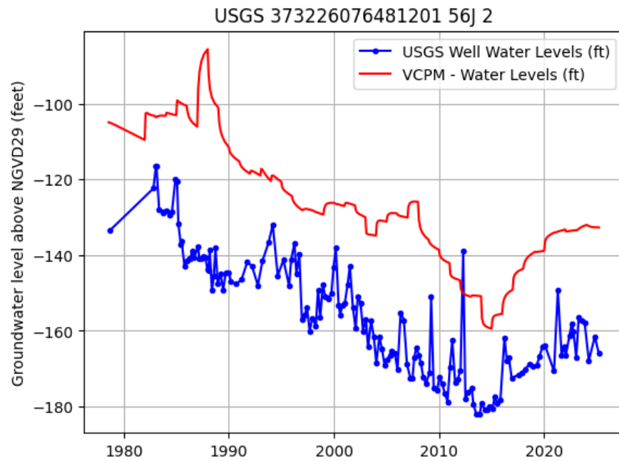
Figure 3. USGS Regional Observation Well 56J 2, None water levels (Potomac Group) recorded from 1978 to present (well depth 600.0 ft bls, land surface 25.0 ft msl) and VAHydroGW-VCPM reported use water levels.
