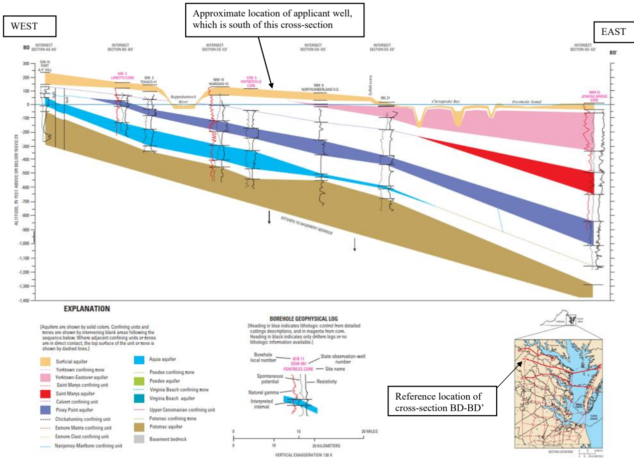
Coastal Plain (2006) Cross-Section BD-BD' from USGS Professional Paper 1731.
