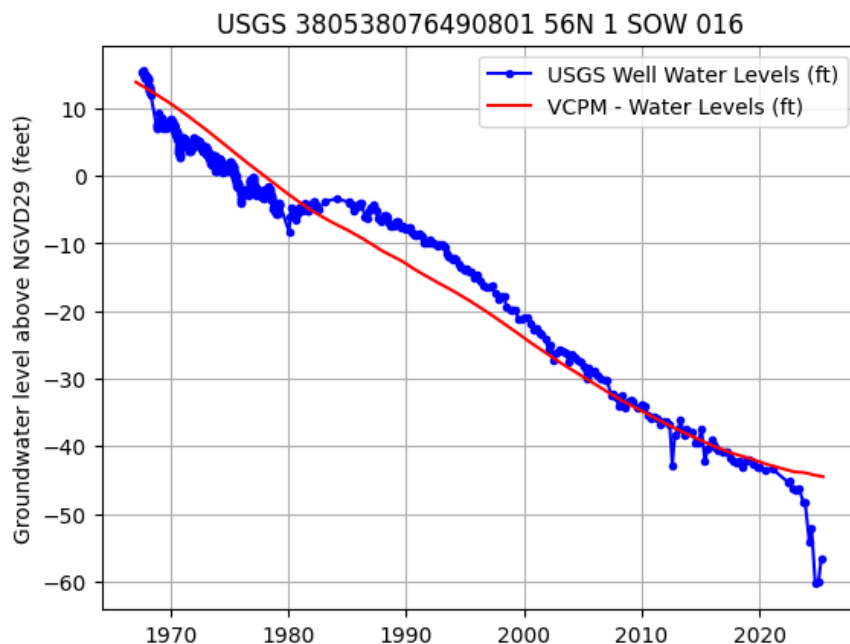
Figure 2. USGS Regional Observation Well 56N 1 SOW 016, Potomac Aquifer water levels (Upper Cretaceous Series) recorded from 1967 to present (well depth 641.0 ft bls, land surface 149.0 ft msl) and VAHydroGW-VCPM reported use water levels.
