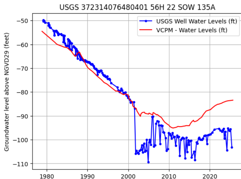
Figure 3. USGS Regional Observation Well 56H 22 SOW 135A, Potomac Aquifer water levels (Patapsco Formation) recorded from 1979 to present (well depth 645.0 ft bls, land surface 105.0 ft msl) and VAHydroGW-VCPM reported use water levels.
