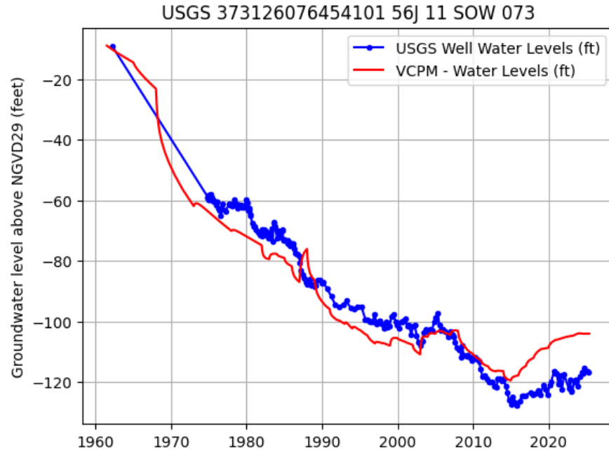
Figure 4. USGS Regional Observation Well 56J 11 SOW 073, Potomac Aquifer water levels (Patuxent Formation) recorded from 1962 to present (well depth 1254.0 ft bls, land surface 15.0 ft msl) and VAHydroGW-VCPM reported use water levels.
