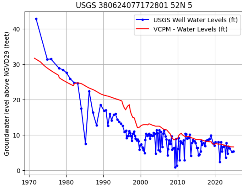
Figure 2. USGS Regional Observation Well 52N 5, Potomac Aquifer water levels (Patapsco Formation) recorded from 1971 to present (well depth 524.0 ft bls, land surface 215.0 ft msl) and VAHydroGW-VCPM reported use water levels.
