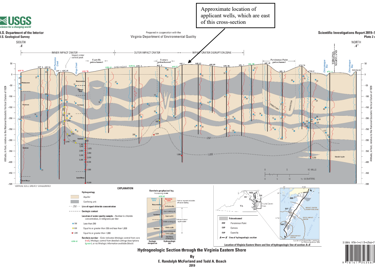
Cross-Section A-A' from USGS Scientific Investigations Report 2019-5093 (2019).
