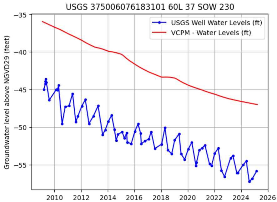
Figure 3. USGS Regional Observation Well 60L 37 SOW 230, Potomac Aquifer water levels (Upper Cretaceous Series) recorded from 2009 to present (well depth 737.31 ft bls, land surface 9.0 ft msl) and VAHydroGW-VCPM reported use water levels.
