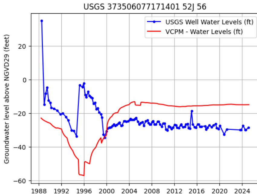
Figure 2. USGS Regional Observation Well 52J 56, Potomac Aquifer water levels (Patapsco Formation) recorded from 1988 to present (well depth 265.0 ft bls, land surface 175.0 ft msl) and VAHydroGW-VCPM reported use water levels.
