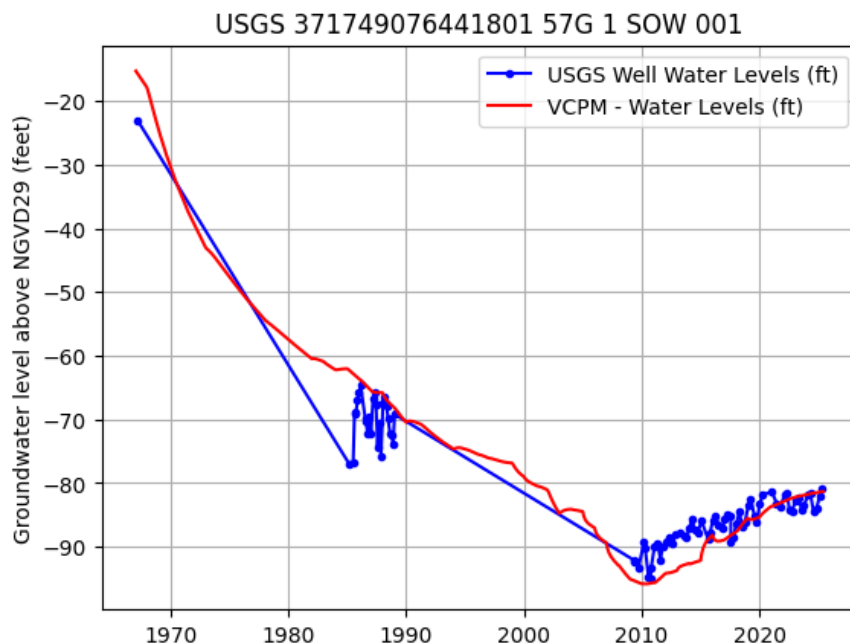
Figure 2. USGS Regional Observation Well 57G 1 SOW 001, Potomac Aquifer water levels (Patapsco Formation) recorded from 1967 to present (well depth 555.0 ft bls, land surface 92.0 ft msl) and VAHydroGW-VCPM reported use water levels.
