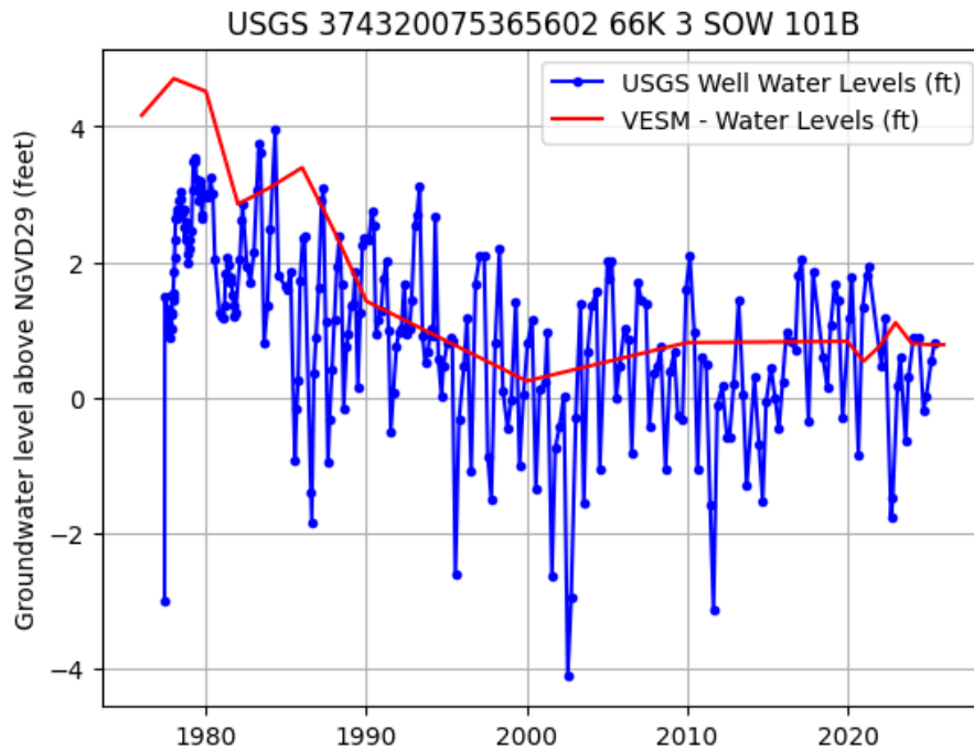
Figure 3. USGS Regional Observation Well 66K 3 SOW 101B, Middle Yorktown-Eastover aquifer water levels recorded from 1977 to present (well depth 222.0 ft bls, land surface 8.0 ft msl) and VAHydroGW-VESM reported use water levels.
