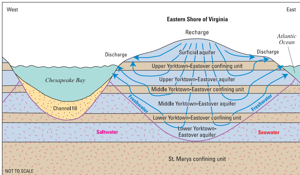
(a) Simplified stratigraphic relations among hydrogeologic units of the Virginia Eastern Shore (adapted from McFarland and Beach, 2019 , and McFarland, 2019 ). Associations among some hydrogeologic units that cross stratigraphic boundaries are not shown. Aquifers, shown in blue, are described in Table 1. The units from the Upper Yorktown-Eastover aquifer to the Lower Yorktown-Eastover aquifer were grouped for the purpose of the regional groundwater budget analysis presented in Section 2.4, below.
