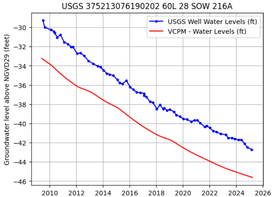
Figure 2. USGS Regional Observation Well 60L 28 SOW 216A, Potomac Aquifer water levels (Patapsco Formation) recorded from 2009 to present (well depth 1224.0 ft bls, land surface 110.0 ft msl) and VAHydroGW-VCPM reported use water levels.
