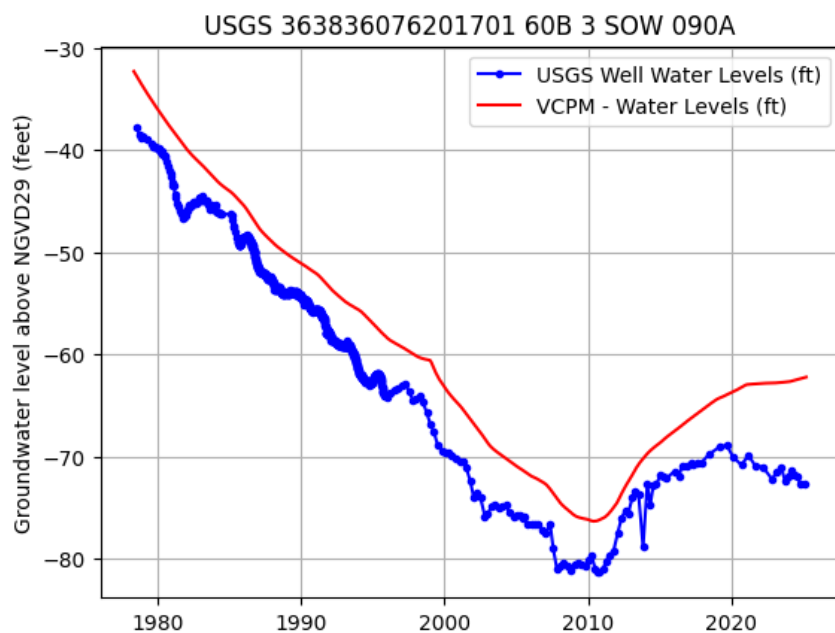
Figure 3. USGS Regional Observation Well 60B 3 SOW 090A, Potomac Aquifer water levels (Upper Cretaceous Series) recorded from 1978 to present (well depth 855.0 ft bls, land surface 16.0 ft msl) and VAHydroGW-VCPM reported use water levels.
